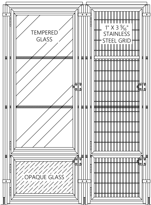
STAINLESS STEEL FRAMED GATES EXAMPLE
