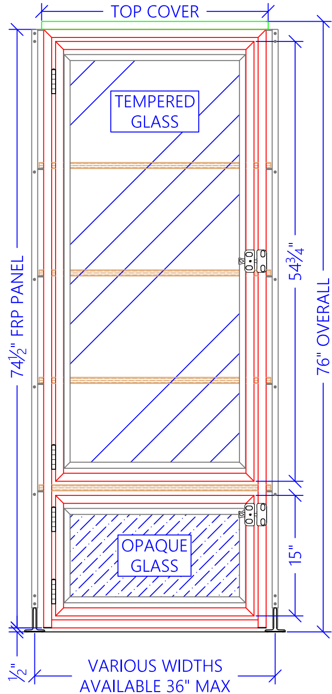
CAT TOWER - FRONT VIEW GLASS GATES
