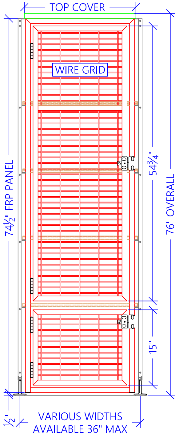
CAT TOWER - FRONT VIEW WIRE GATES
